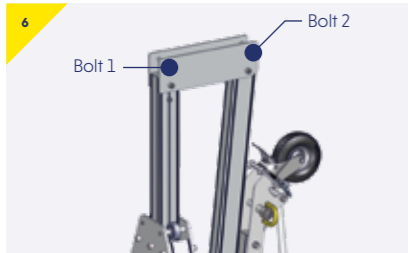
This illustration demonstrates the bolt positions (1 & 2) for the cheek plates.
